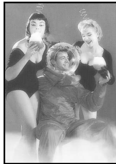
Everything floats without weight after the rocket motors are shut off in space.
